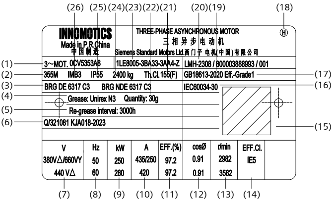
1LE8 铸铁系列电机铭牌 1LE8 Cast iron motor nameplate
